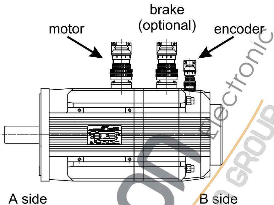
Fig. 7-6: Overview of connections with SB Motor - 1
