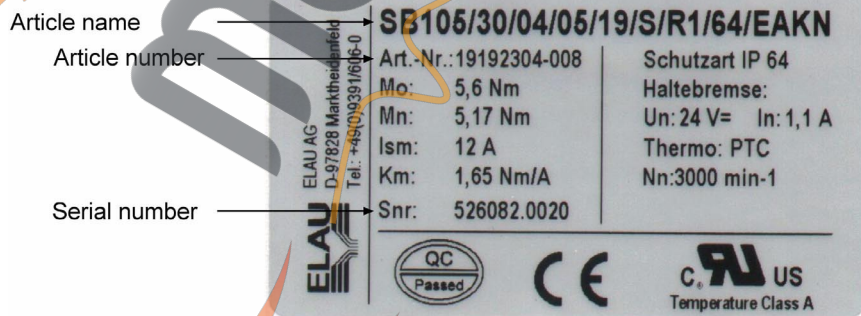
Fig. 5-2: type plate of a SB motors
