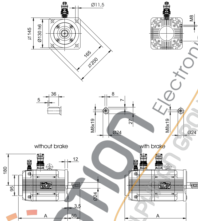
Fig. 7-11: Dimensional drawing of SB 145
